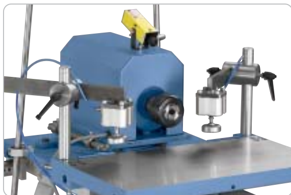
The pneumatic clamping cylinder retrofit the large standard equipment
